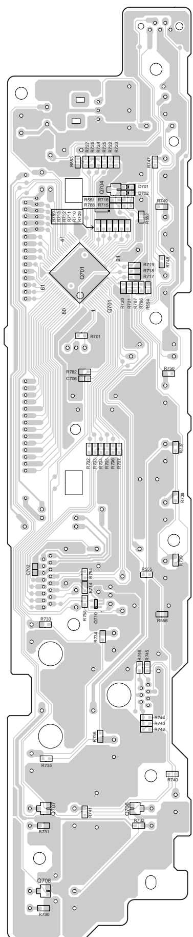
Soldering side view
